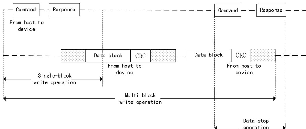
Figure 109 SDIO (Multi-) Data Block Write Operation
