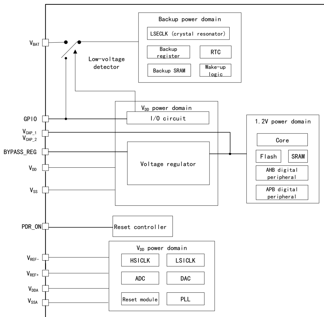
Figure 38 Power Supply Structure Block Diagram
