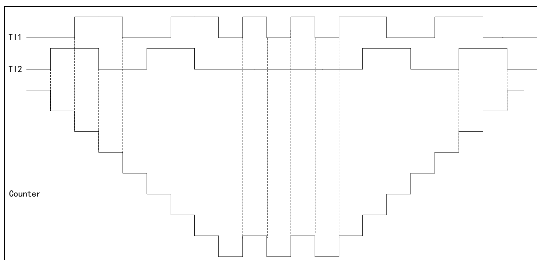
Figure 34 Example of Encoder Interface Mode of IC1FP1 Reversed Phase
