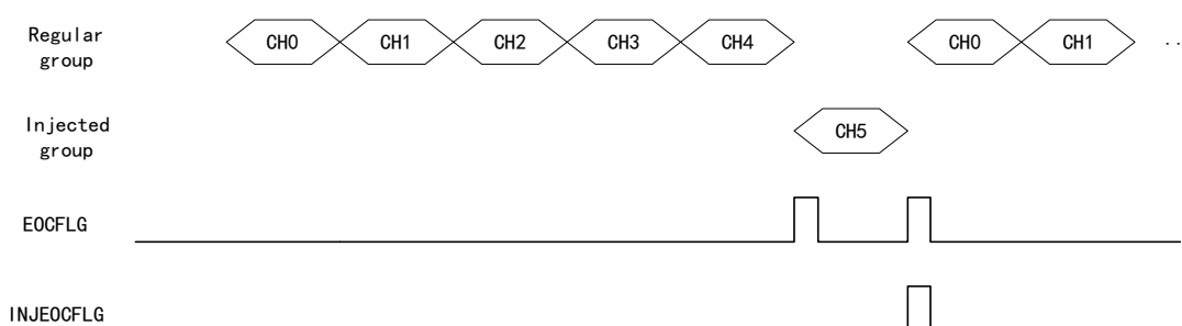
Figure 119 Automatic Injection Timing Diagram
