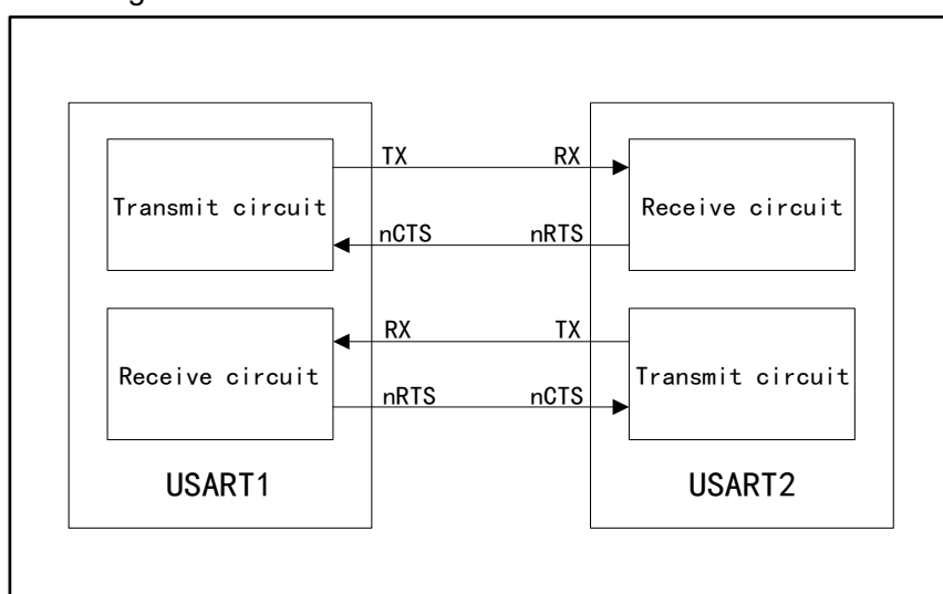
Figure 76 Hardware Flow Control between Two USART
