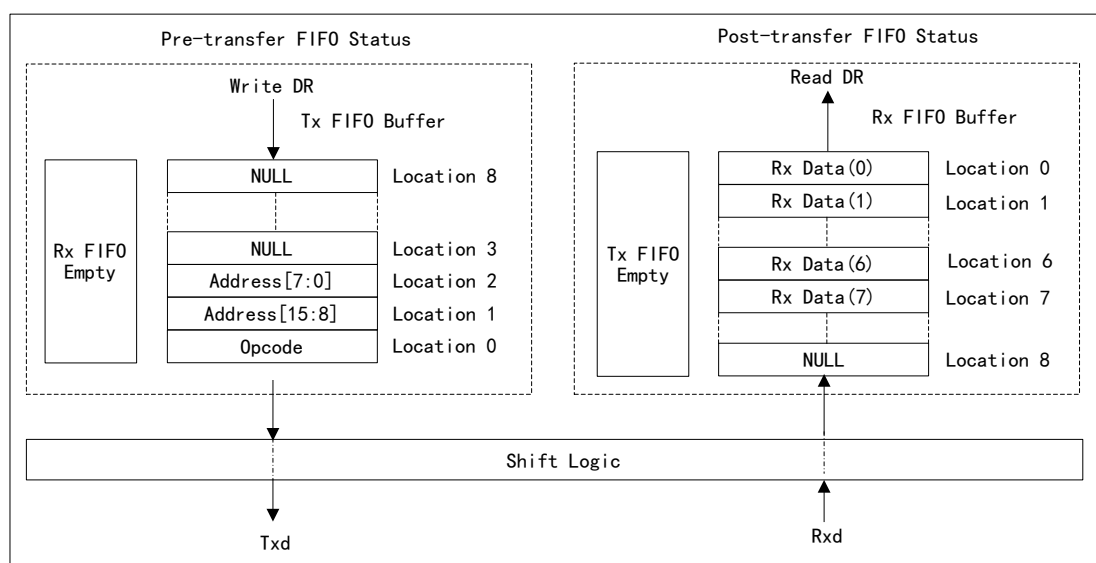
Figure 93 FIFO Status in EEPROM Read Transfer Mode
